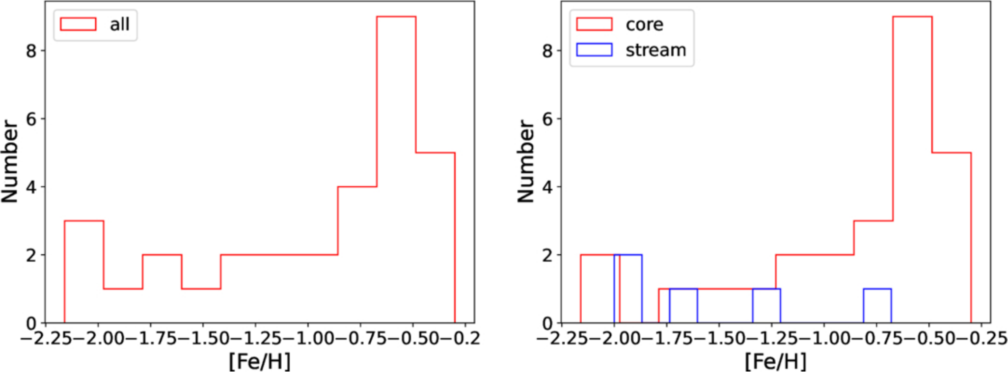
Figure 6. from P. Wang et al 2026 Astron. J. 172 doi:10.3847/1538-3881/ae81b5 https://dx.doi.org/10.3847/1538-3881/ae81b5 © 2026. The Author(s). Published by the American Astronomical Society.
