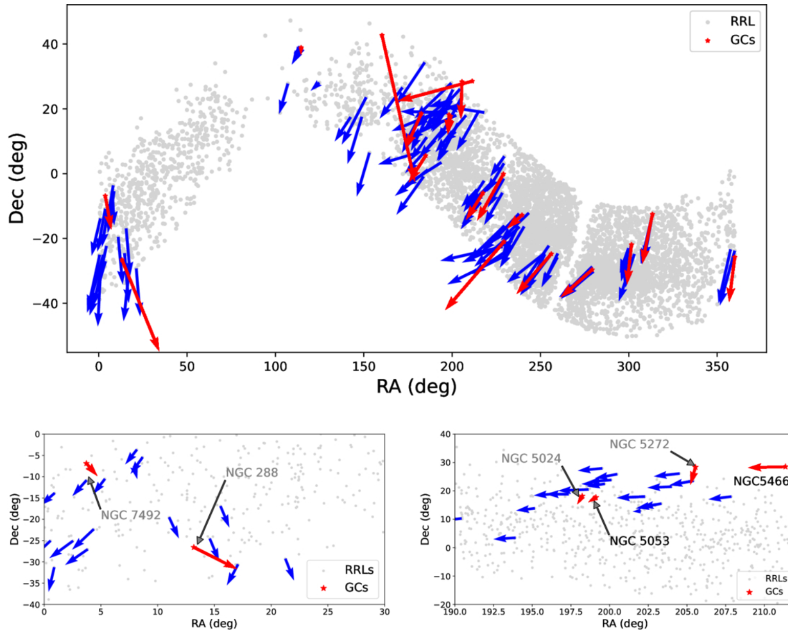
Figure 4. from P. Wang et al 2026 Astron. J. 172 doi:10.3847/1538-3881/ae81b5 https://dx.doi.org/10.3847/1538-3881/ae81b5 © 2026. The Author(s). Published by the American Astronomical Society.
