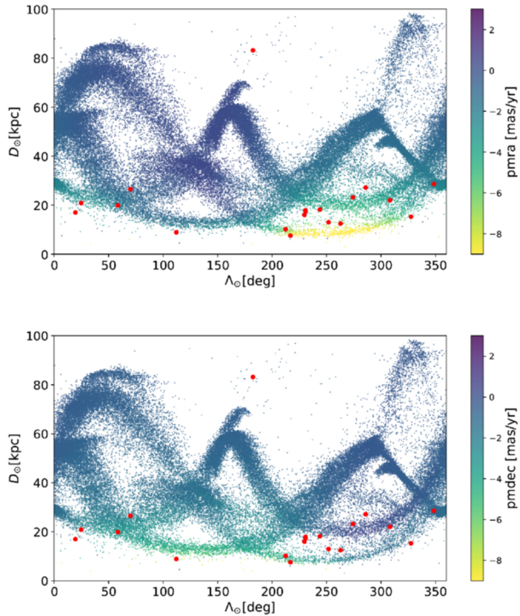
Figure 3. from P. Wang et al 2026 Astron. J. 172 doi:10.3847/1538-3881/ae81b5 https://dx.doi.org/10.3847/1538-3881/ae81b5 © 2026. The Author(s). Published by the American Astronomical Society.
