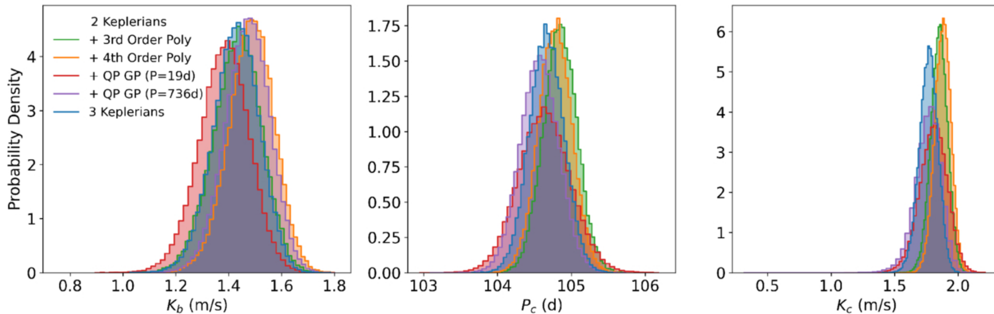
Figure 4. from Victoria DiTomaso et al 2026 Astron. J. 172 doi:10.3847/1538-3881/ae819f https://dx.doi.org/10.3847/1538-3881/ae819f © 2026. The Author(s). Published by the American Astronomical Society.
