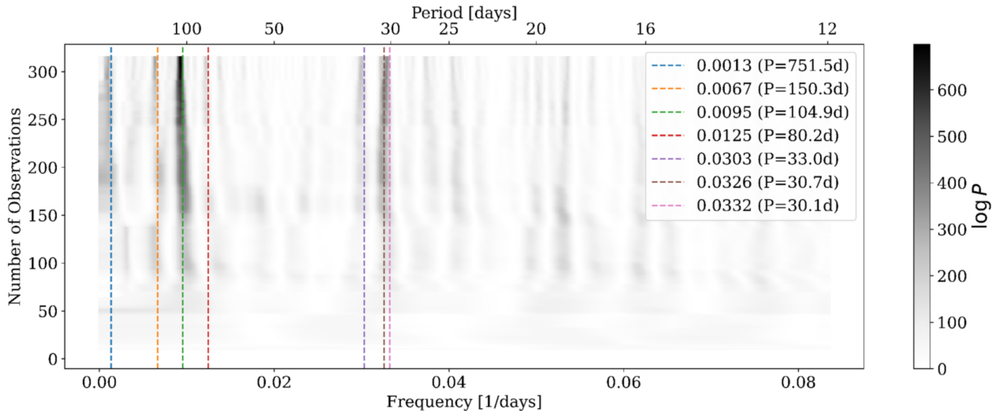
Figure 3. from Victoria DiTomasso et al 2026 Astron. J. 172 doi:10.3847/1538-3881/ae819f https://dx.doi.org/10.3847/1538-3881/ae819f © 2026. The Author(s). Published by the American Astronomical Society.
