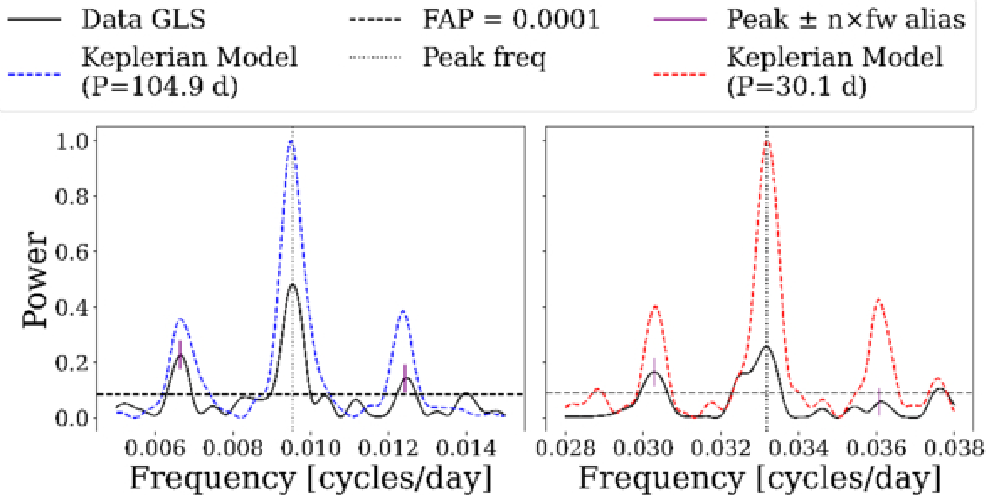
Figure 2. from Victoria DiTomaso et al 2026 Astron. J. 172 doi:10.3847/1538-3881/ae819f https://dx.doi.org/10.3847/1538-3881/ae819f © 2026. The Author(s). Published by the American Astronomical Society.
