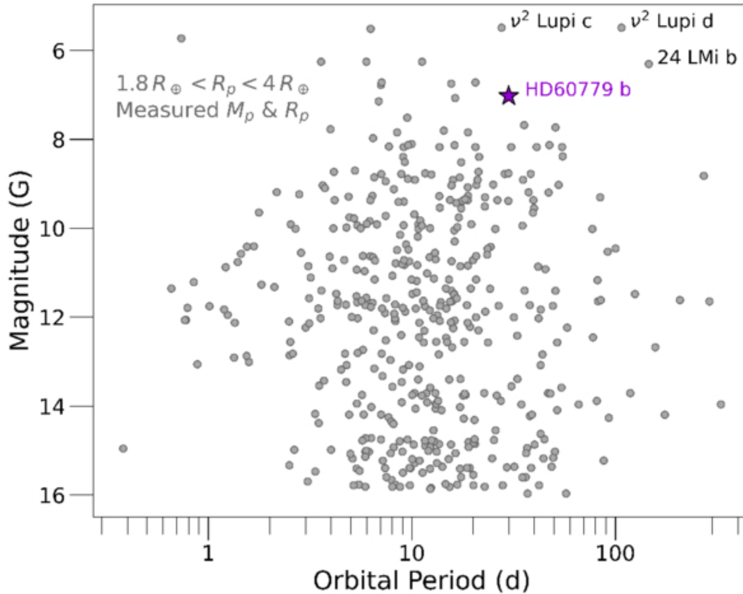
Figure 10. from Victoria DiTomaso et al 2026 Astron. J. 172 doi:10.3847/1538-3881/ae819f https://dx.doi.org/10.3847/1538-3881/ae819f © 2026. The Author(s). Published by the American Astronomical Society.
