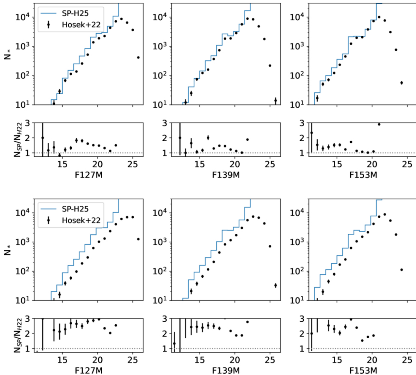
Figure 7. from Macy J. Huston et al 2026 Astron. J. 172 doi:10.3847/1538-3881/ae8156 https://dx.doi.org/10.3847/1538-3881/ae8156 © 2026. The Author(s). Published by the American Astronomical Society.
