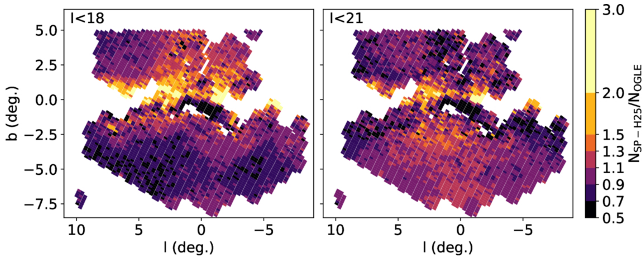
Figure 4. from Macy J. Huston et al 2026 Astron. J. 172 doi:10.3847/1538-3881/ae8156 https://dx.doi.org/10.3847/1538-3881/ae8156 © 2026. The Author(s). Published by the American Astronomical Society.
