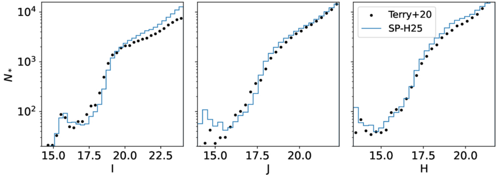
Figure 3. from Macy J. Huston et al 2026 Astron. J. 172 doi:10.3847/1538-3881/ae8156 https://dx.doi.org/10.3847/1538-3881/ae8156 © 2026. The Author(s). Published by the American Astronomical Society.
