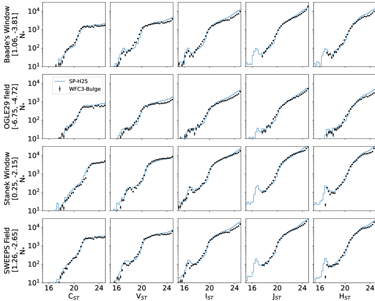
Figure 2. from Macy J. Huston et al 2026 Astron. J. 172 doi:10.3847/1538-3881/ae8156 https://dx.doi.org/10.3847/1538-3881/ae8156 © 2026. The Author(s). Published by the American Astronomical Society.
