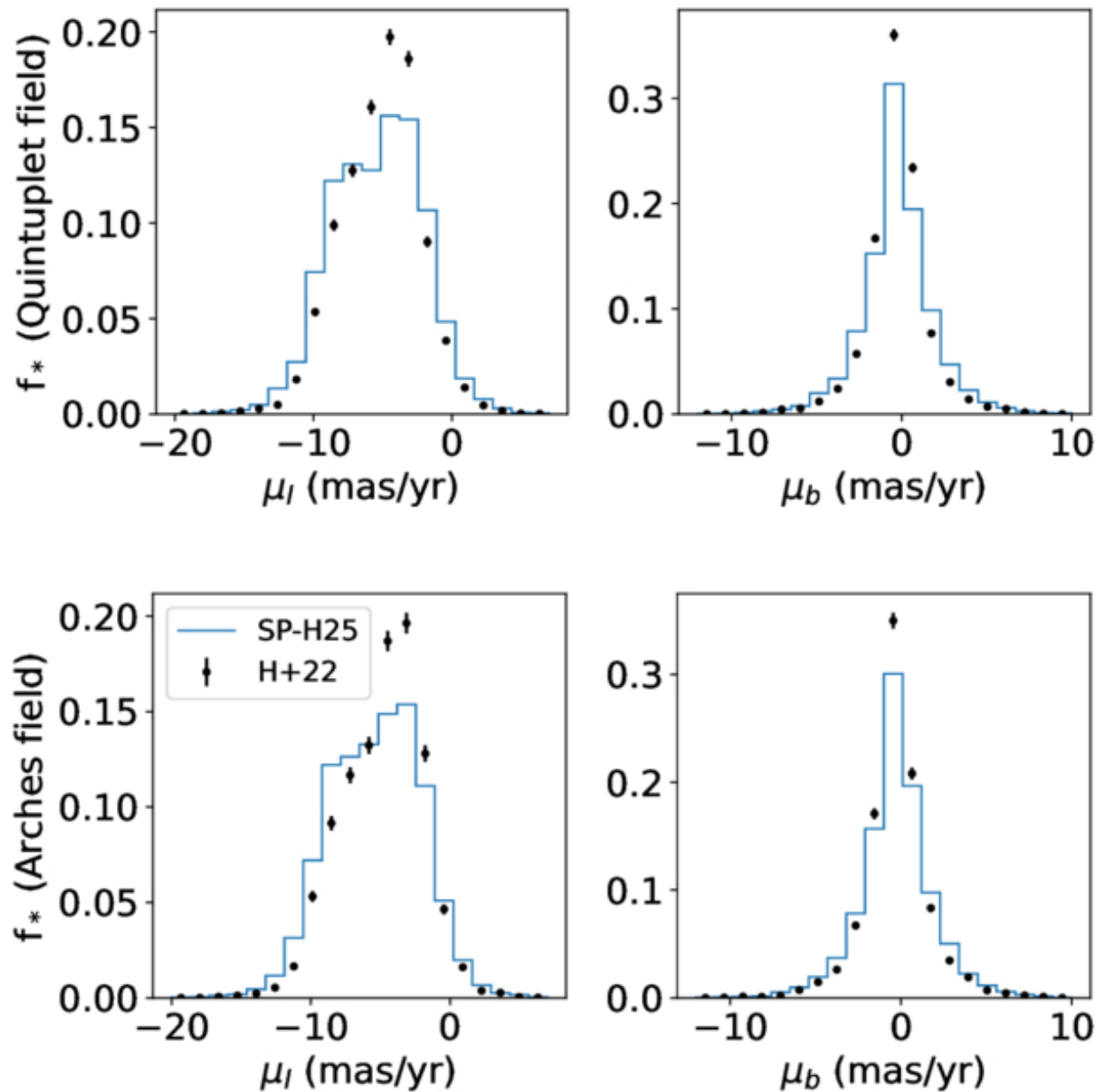
Figure 10. from Macy J. Huston et al 2026 Astron. J. 172 doi:10.3847/1538-3881/ae8156 https://dx.doi.org/10.3847/1538-3881/ae8156 © 2026. The Author(s). Published by the American Astronomical Society.
