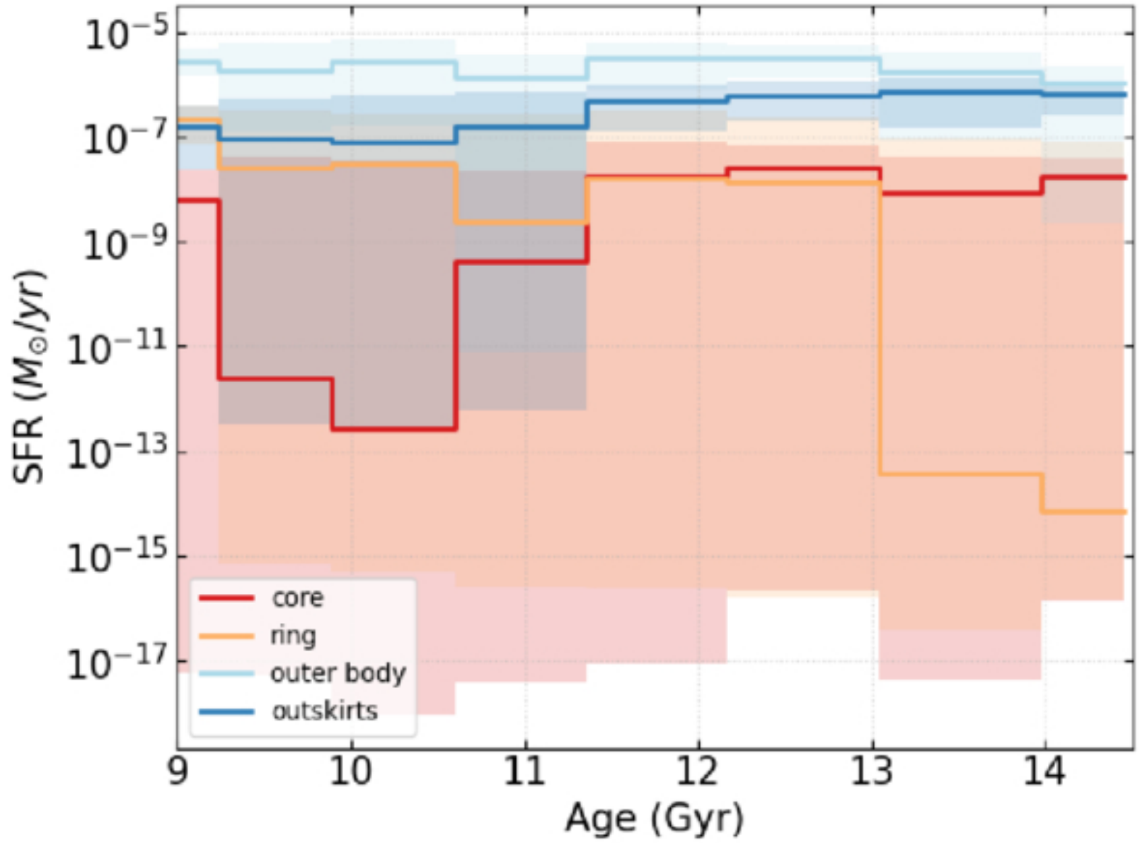
Figure 5. from Andrés E. Piatti 2026 Astron. J. 172 doi:10.3847/1538-3881/ae80c1 https://dx.doi.org/10.3847/1538-3881/ae80c1 © 2026. The Author(s). Published by the American Astronomical Society.
