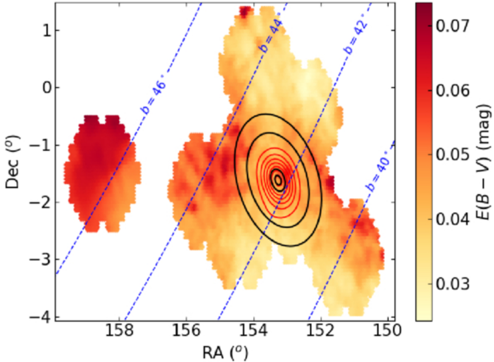
Figure 1. from Andrés E. Piatti 2026 Astron. J. 172 doi:10.3847/1538-3881/ae80c1 https://dx.doi.org/10.3847/1538-3881/ae80c1 © 2026. The Author(s). Published by the American Astronomical Society.
