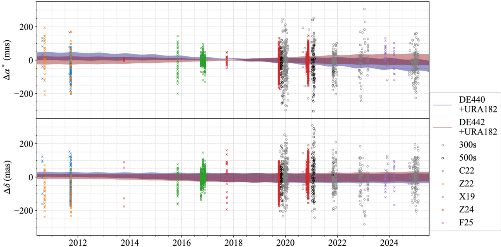
Figure 8. from Jian Chen et al 2026 Astron. J. 172 doi:10.3847/1538-3881/ae8096 https://dx.doi.org/10.3847/1538-3881/ae8096 © 2026. The Author(s). Published by the American Astronomical Society.
