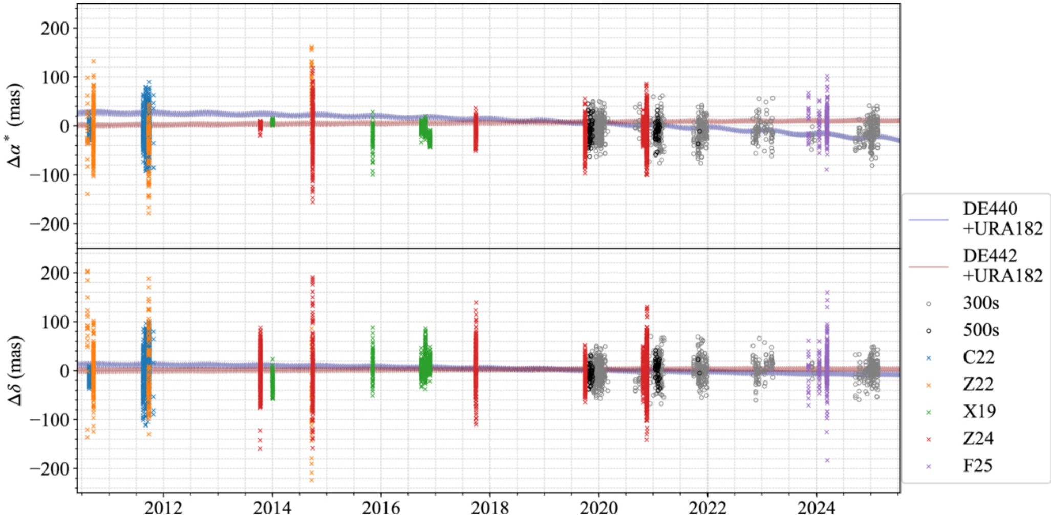
Figure 7. from Jian Chen et al 2026 Astron. J. 172 doi:10.3847/1538-3881/ae8096 https://dx.doi.org/10.3847/1538-3881/ae8096 © 2026. The Author(s). Published by the American Astronomical Society.
