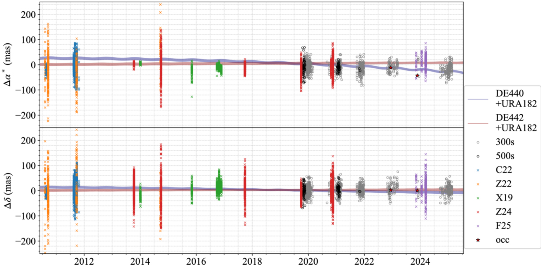
Figure 6. from Jian Chen et al 2026 Astron. J. 172 doi:10.3847/1538-3881/ae8096 https://dx.doi.org/10.3847/1538-3881/ae8096 © 2026. The Author(s). Published by the American Astronomical Society.
