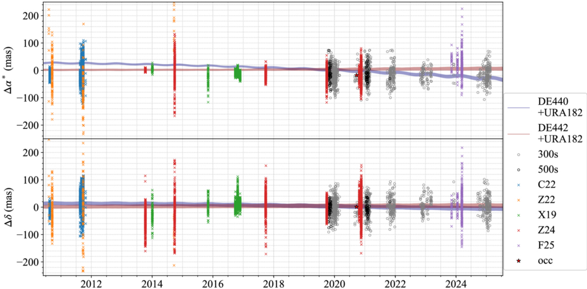
Figure 5. from Jian Chen et al 2026 Astron. J. 172 doi:10.3847/1538-3881/ae8096 https://dx.doi.org/10.3847/1538-3881/ae8096 © 2026. The Author(s). Published by the American Astronomical Society.
