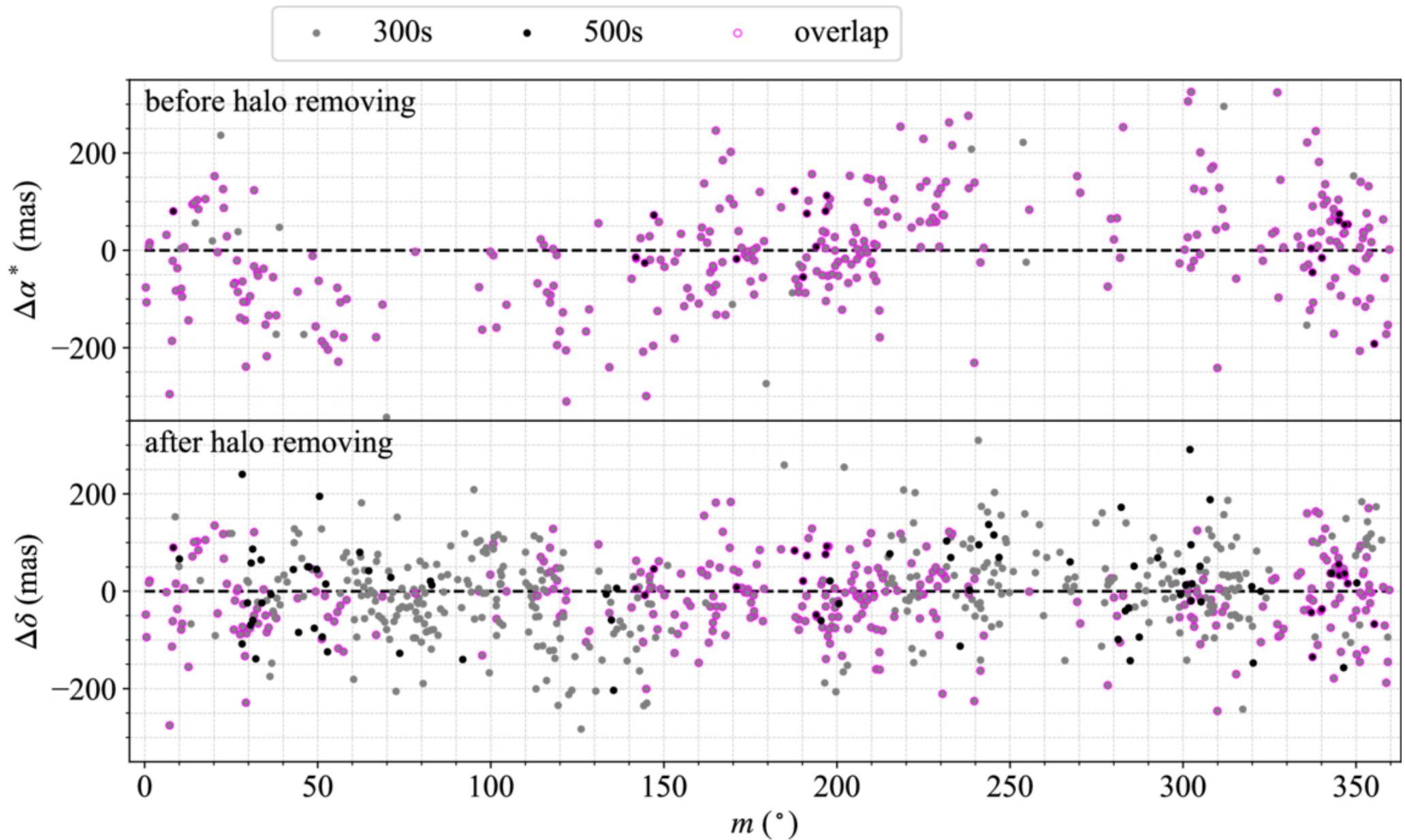
Figure 3. from Jian Chen et al 2026 Astron. J. 172 doi:10.3847/1538-3881/ae8096 https://dx.doi.org/10.3847/1538-3881/ae8096 © 2026. The Author(s). Published by the American Astronomical Society.
