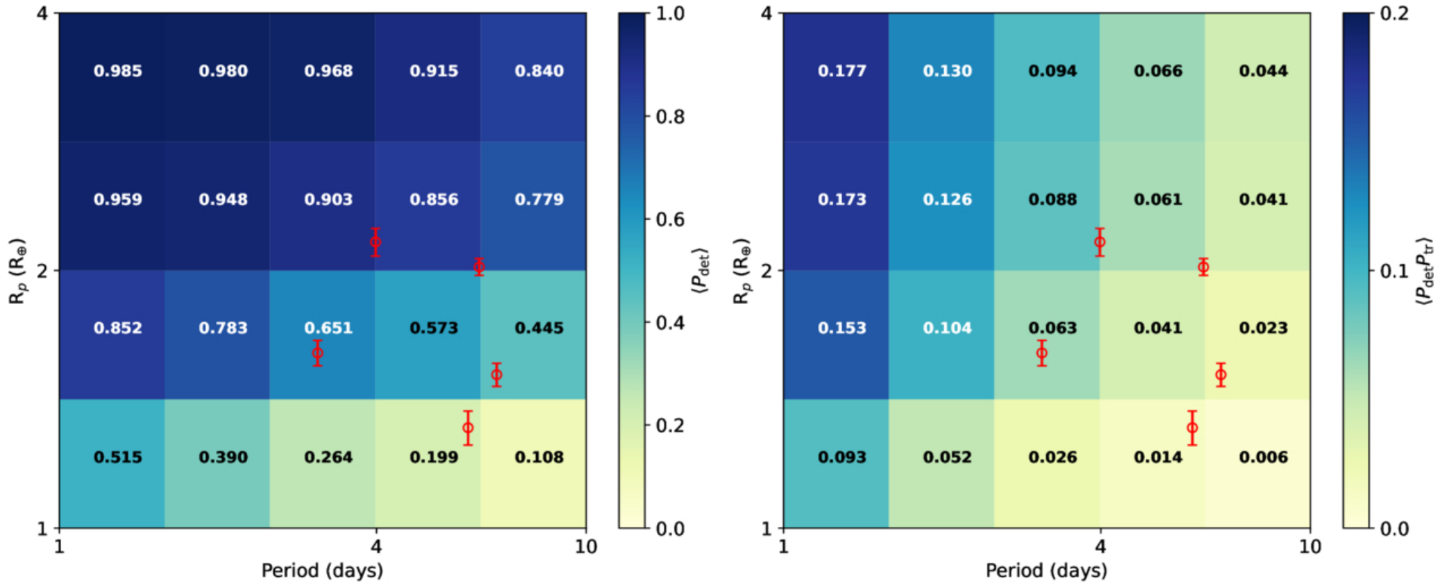
Figure 3. from Quanyi Liu et al 2026 Astron. J. 172 doi:10.3847/1538-3881/ae7deb https://dx.doi.org/10.3847/1538-3881/ae7deb © 2026. The Author(s). Published by the American Astronomical Society.
