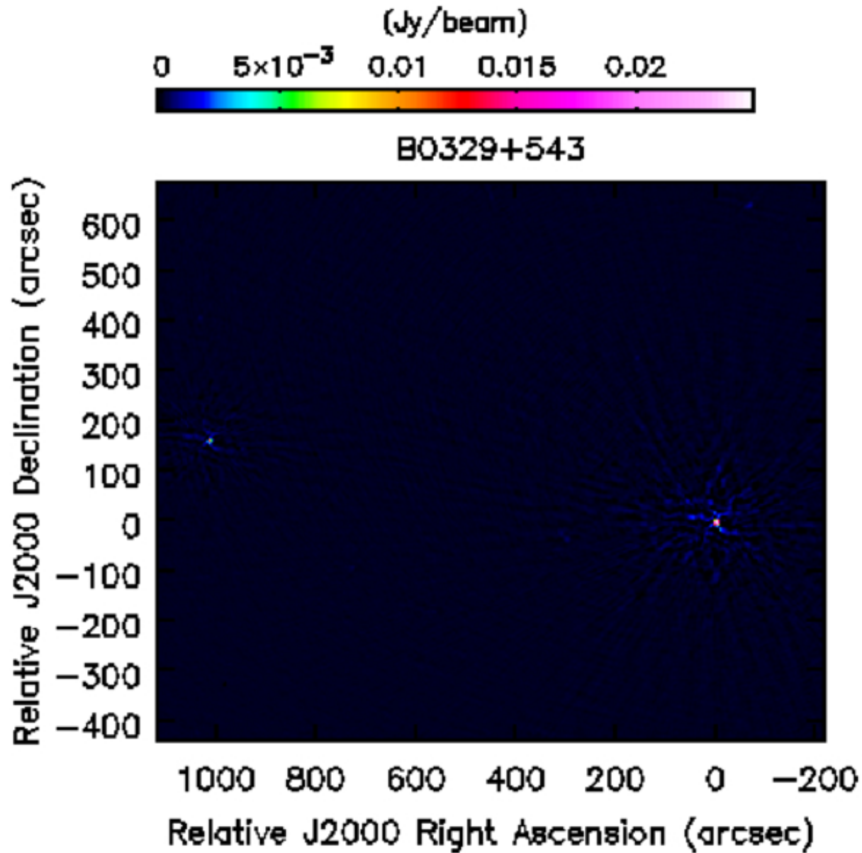
Figure 4. from Jitendra Salal et al 2026 Astron. J. 172 doi:10.3847/1538-3881/ae7d11 https://dx.doi.org/10.3847/1538-3881/ae7d11 © 2026. The Author(s). Published by the American Astronomical Society.
