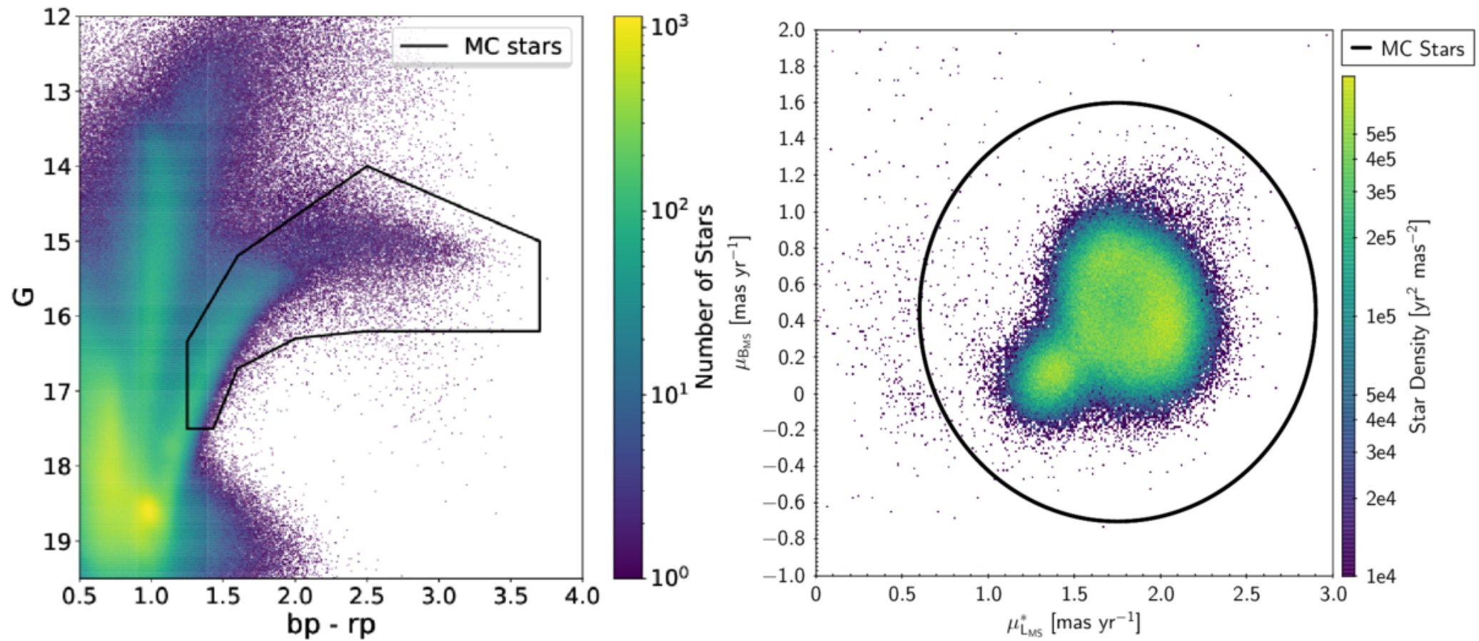
Figure 9. from David L. Nidever et al 2026 Astron. J. 172 doi:10.3847/1538-3881/ae7c76 https://dx.doi.org/10.3847/1538-3881/ae7c76 © 2026. The Author(s). Published by the American Astronomical Society.
