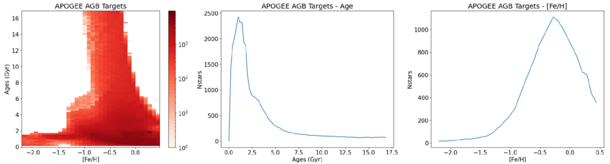
Figure 8. from David L. Nidever et al 2026 Astron. J. 172 doi:10.3847/1538-3881/ae7c76 https://dx.doi.org/10.3847/1538-3881/ae7c76 © 2026. The Author(s). Published by the American Astronomical Society.
