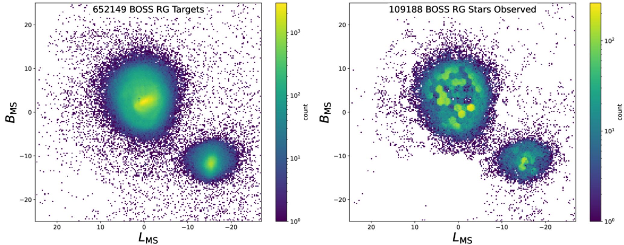
Figure 5. from David L. Nidever et al 2026 Astron. J. 172 doi:10.3847/1538-3881/ae7c76 https://dx.doi.org/10.3847/1538-3881/ae7c76 © 2026. The Author(s). Published by the American Astronomical Society.
