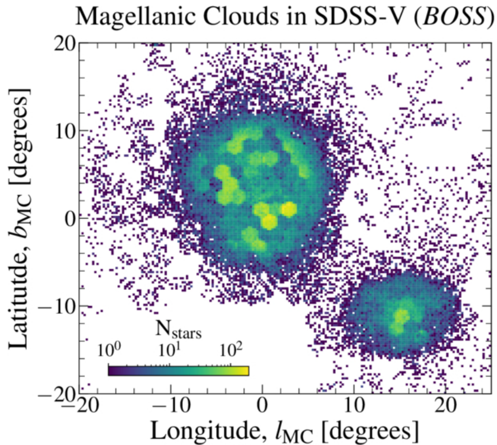
Figure 2. from David L. Nidever et al 2026 Astron. J. 172 doi:10.3847/1538-3881/ae7c76 https://dx.doi.org/10.3847/1538-3881/ae7c76 © 2026. The Author(s). Published by the American Astronomical Society.
