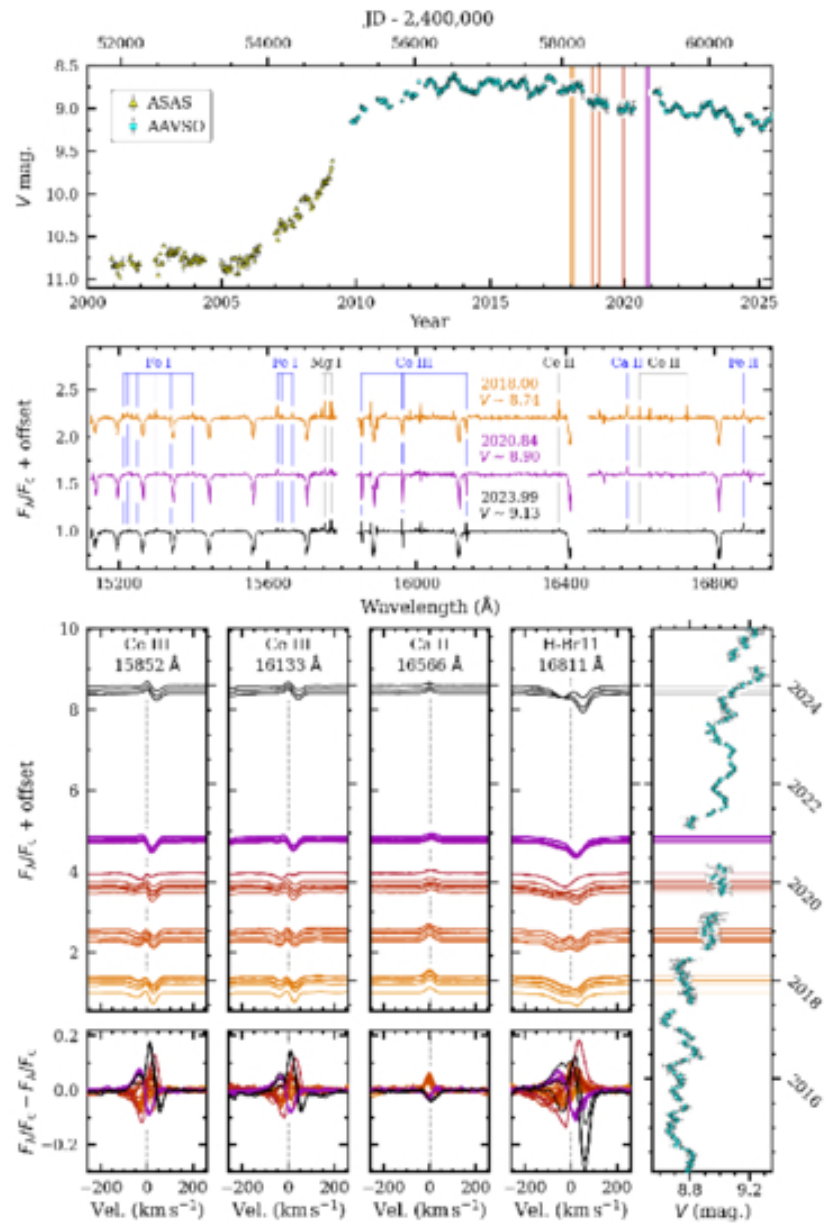
Figure 17. from David L. Nidever et al 2026 Astron. J. 172 doi:10.3847/1538-3881/ae7c76 https://dx.doi.org/10.3847/1538-3881/ae7c76 © 2026. The Author(s). Published by the American Astronomical Society.
