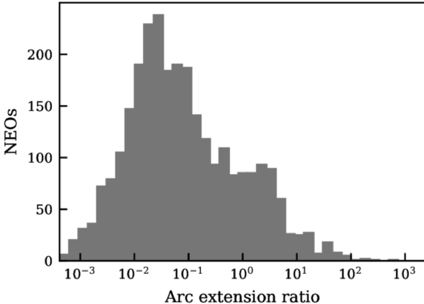
Figure 3. from Sage Li et al 2026 Astron. J. 172 doi:10.3847/1538-3881/ae7c73 https://dx.doi.org/10.3847/1538-3881/ae7c73 © 2026. The Author(s). Published by the American Astronomical Society.
