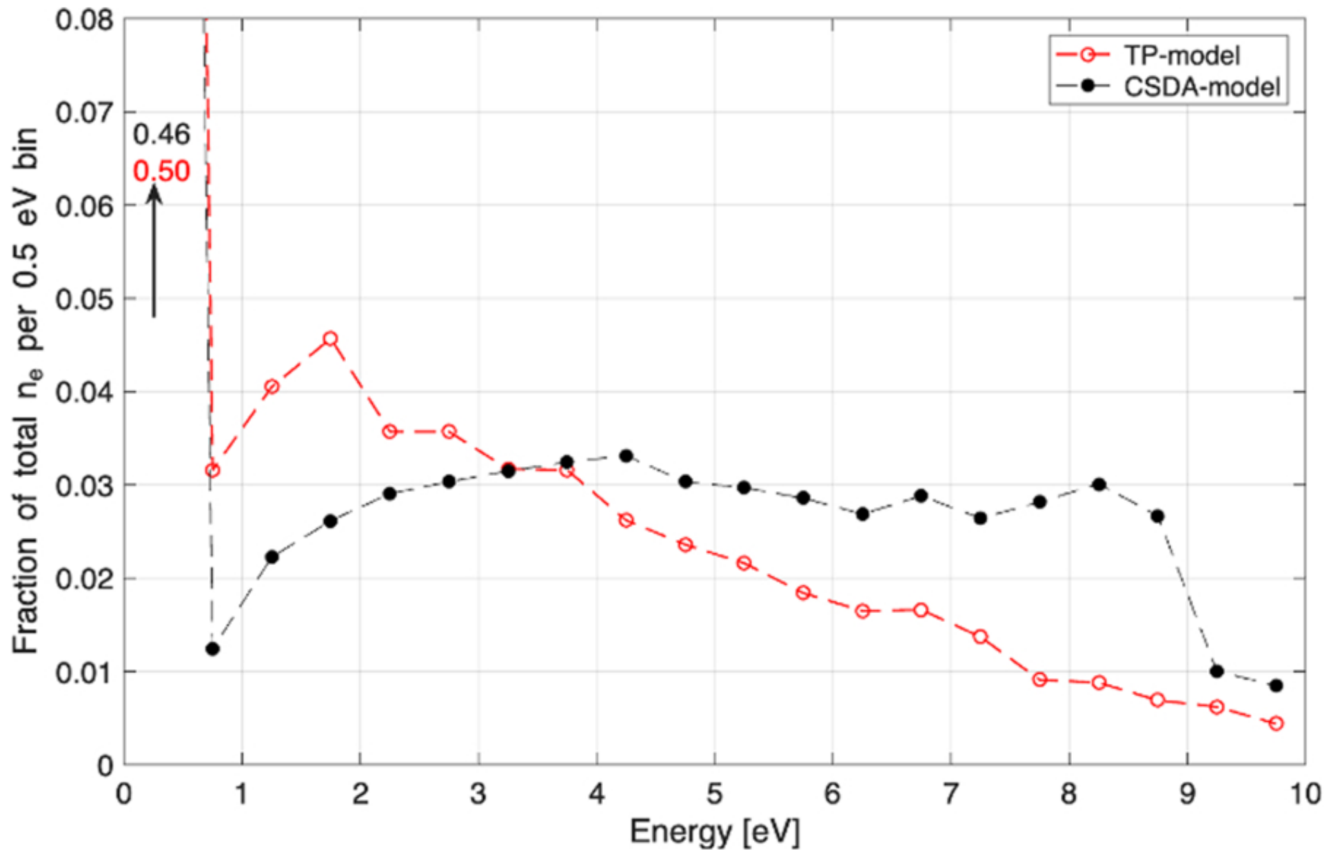
Figure 2. from Erik Vigren and Anders I. Eriksson 2026 Astron. J. 172 doi:10.3847/1538-3881/ae7beb https://dx.doi.org/10.3847/1538-3881/ae7beb © 2026. The Author(s). Published by the American Astronomical Society.
