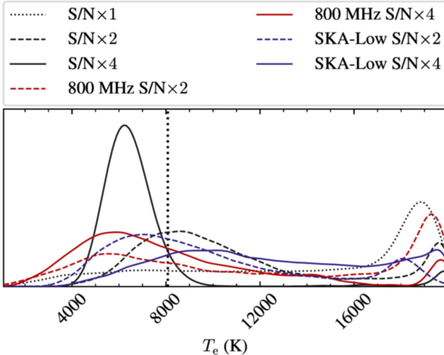
Figure 8. from Pedro Salas et al 2026 Astron. J. 172 doi:10.3847/1538-3881/ae7a69 https://dx.doi.org/10.3847/1538-3881/ae7a69 © 2026. The Author(s). Published by the American Astronomical Society.
