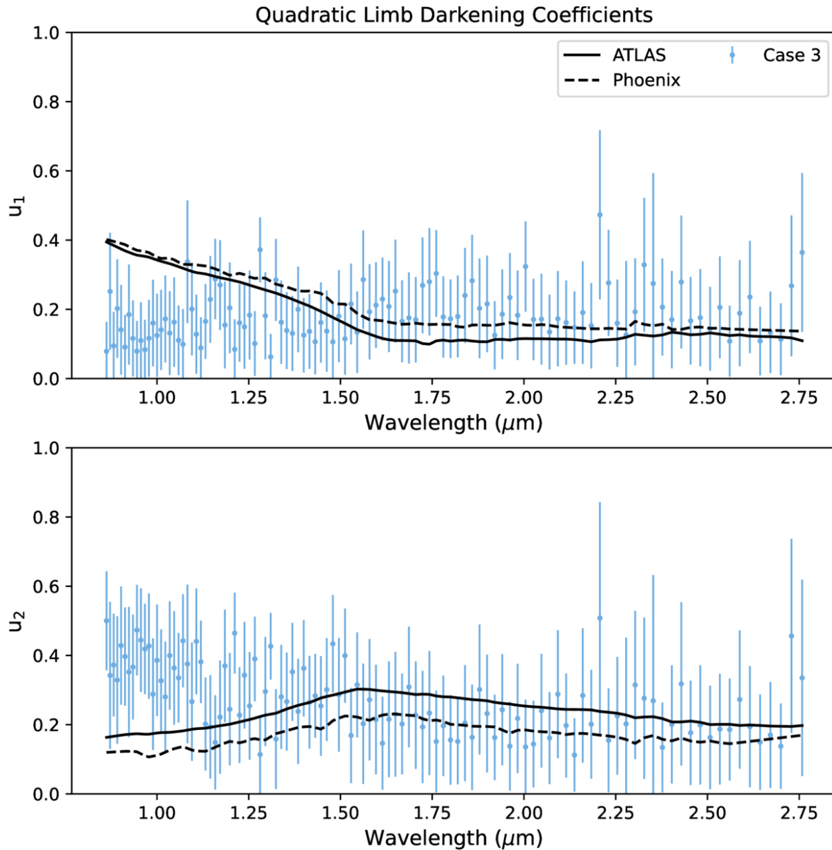
Figure 13. from Matthew M. Murphy et al 2026 Astron. J. 172 doi:10.3847/1538-3881/ae7a32 https://dx.doi.org/10.3847/1538-3881/ae7a32 © 2026. The Author(s). Published by the American Astronomical Society.
