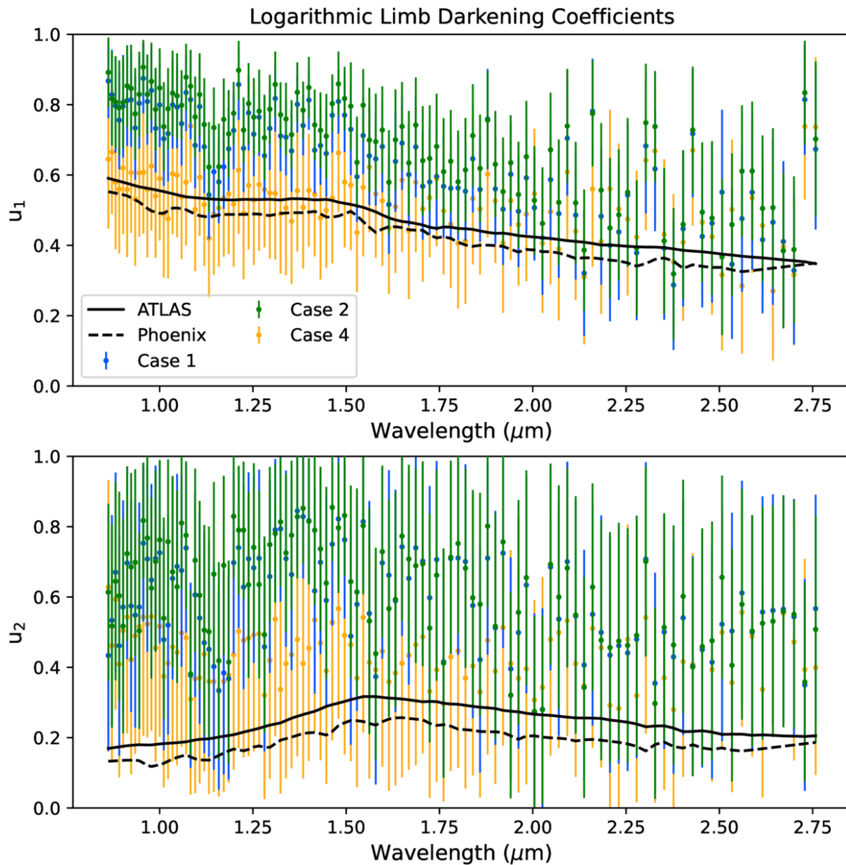
Figure 12. from Matthew M. Murphy et al 2026 Astron. J. 172 doi:10.3847/1538-3881/ae7a32 https://dx.doi.org/10.3847/1538-3881/ae7a32 © 2026. The Author(s). Published by the American Astronomical Society.
