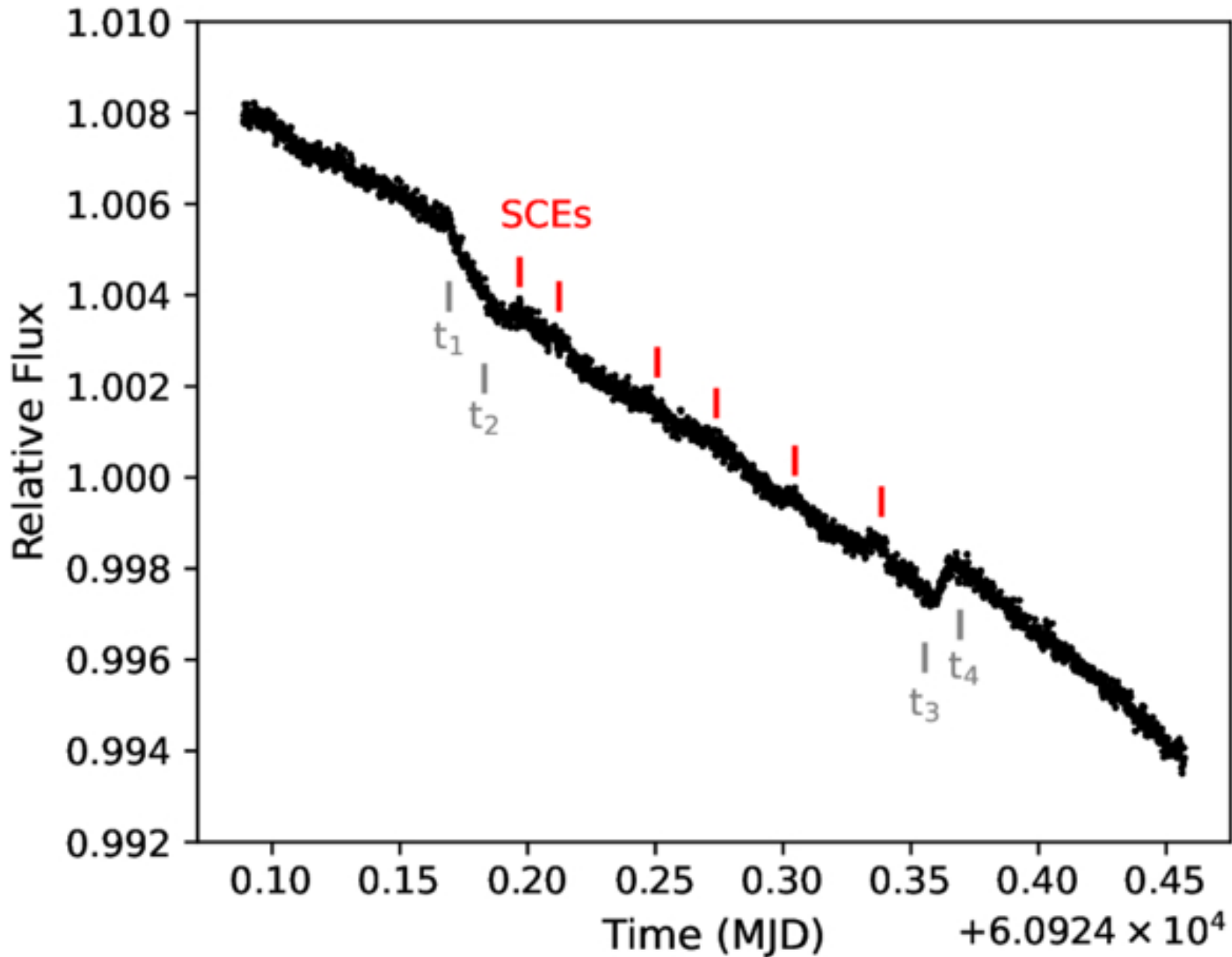
Figure 1. from Matthew M. Murphy et al 2026 Astron. J. 172 doi:10.3847/1538-3881/ae7a32 https://dx.doi.org/10.3847/1538-3881/ae7a32 © 2026. The Author(s). Published by the American Astronomical Society.
