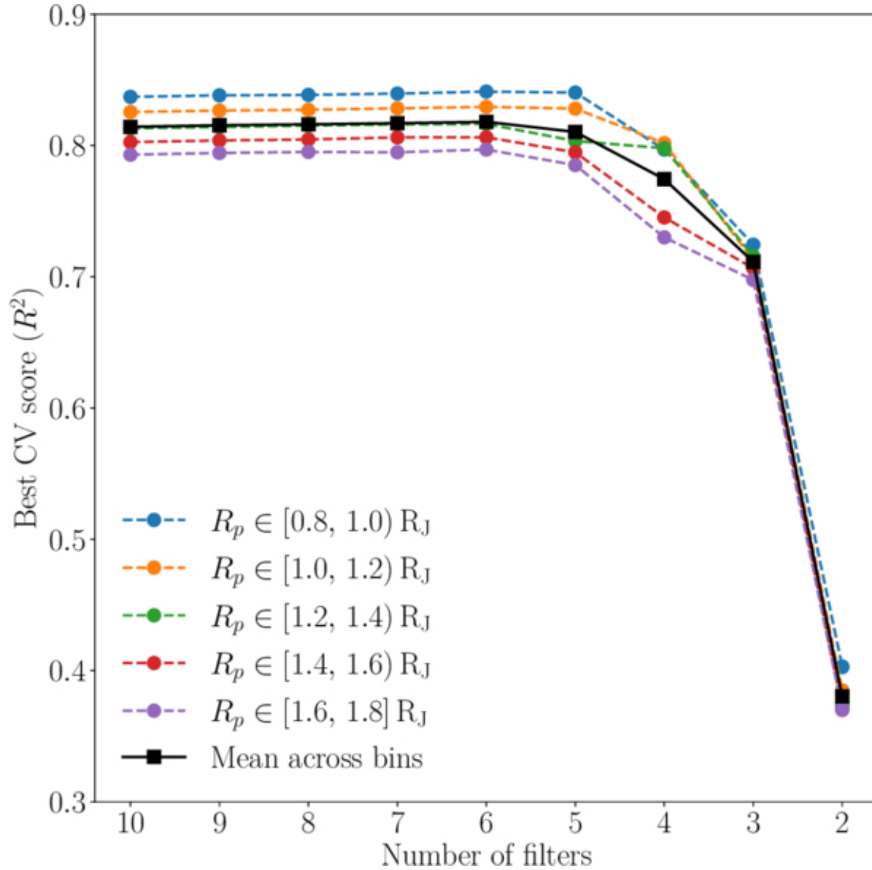
Figure 9. from Patcharawee Munsaket et al 2026 Astron. J. 172 doi:10.3847/1538-3881/ae78df https://dx.doi.org/10.3847/1538-3881/ae78df © 2026. The Author(s). Published by the American Astronomical Society.
