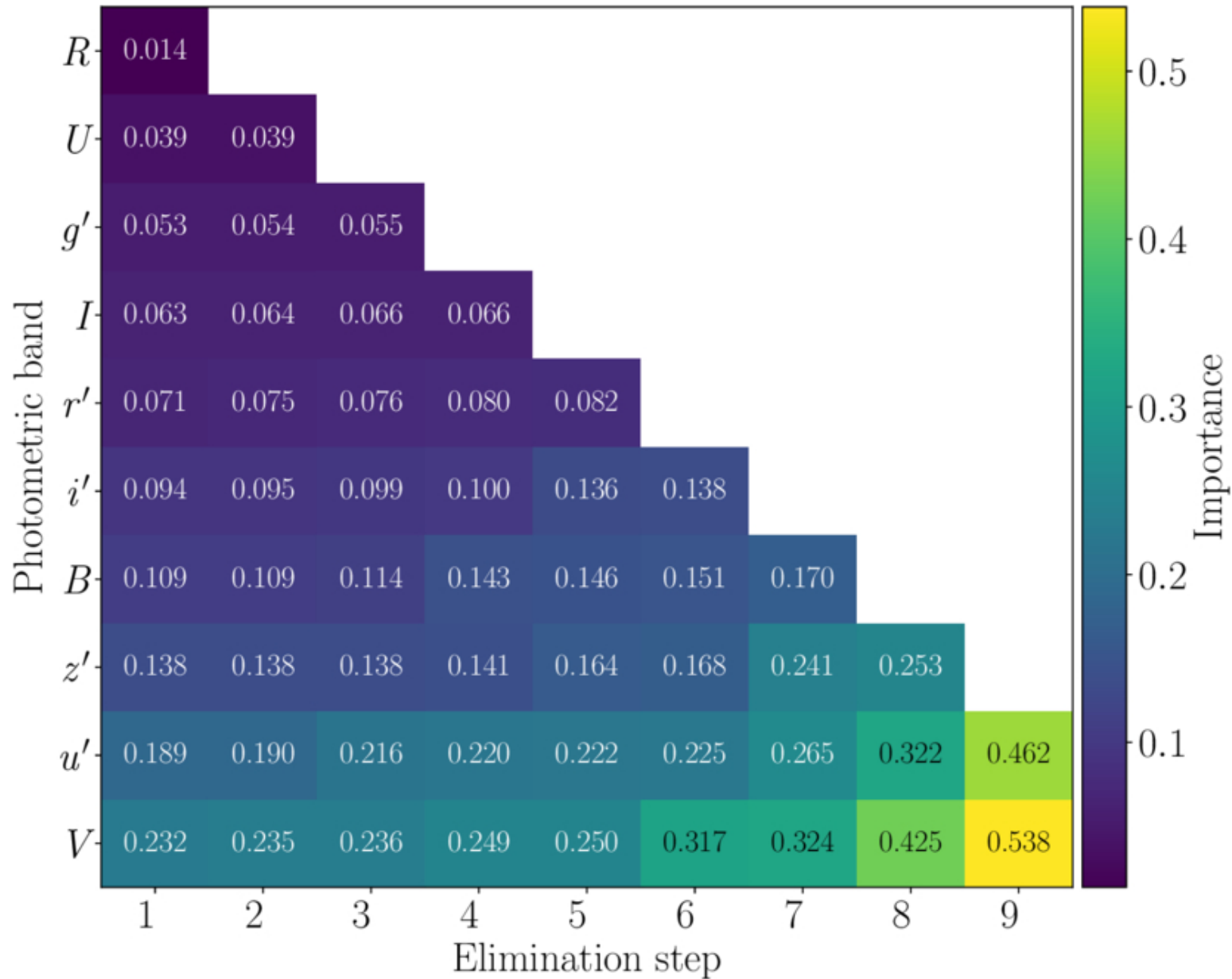
Figure 8. from Patcharawee Munsaket et al 2026 Astron. J. 172 doi:10.3847/1538-3881/ae78df https://dx.doi.org/10.3847/1538-3881/ae78df © 2026. The Author(s). Published by the American Astronomical Society.
