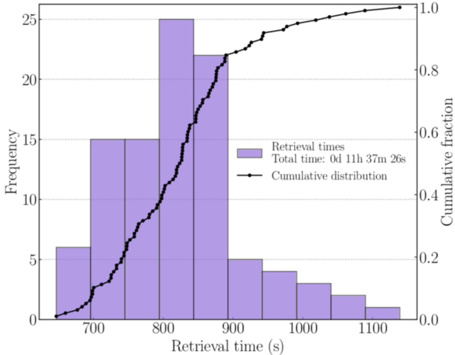
Figure 6. from Patcharawee Munsaket et al 2026 Astron. J. 172 doi:10.3847/1538-3881/ae78df https://dx.doi.org/10.3847/1538-3881/ae78df © 2026. The Author(s). Published by the American Astronomical Society.
