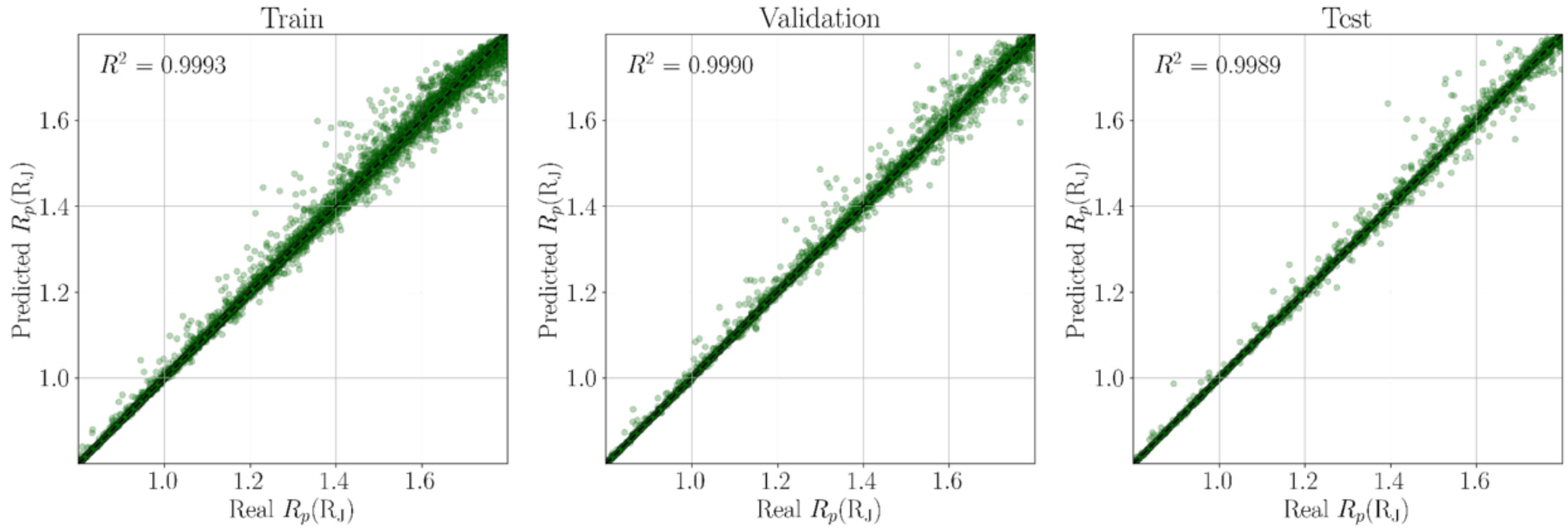
Figure 3. from Patcharawee Munsaket et al 2026 Astron. J. 172 doi:10.3847/1538-3881/ae78df https://dx.doi.org/10.3847/1538-3881/ae78df © 2026. The Author(s). Published by the American Astronomical Society.
