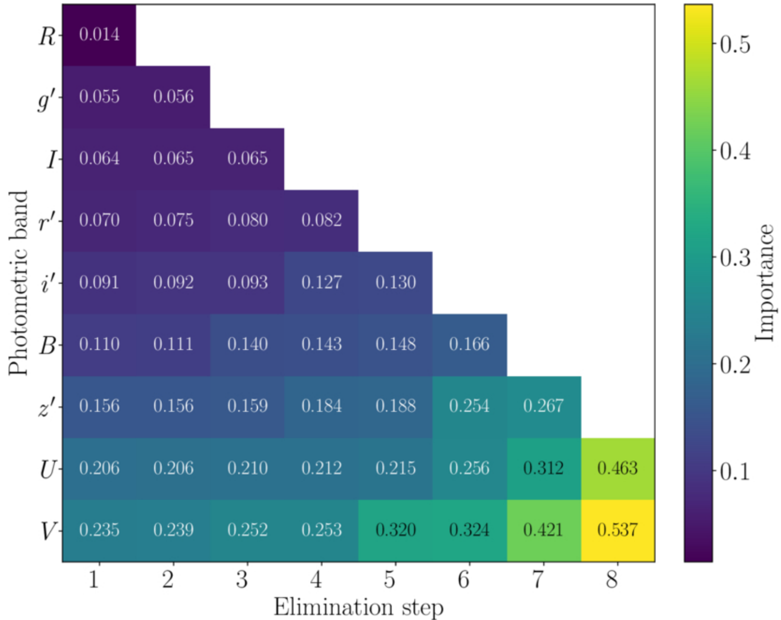
Figure 12. from Patcharawee Munsaket et al 2026 Astron. J. 172 doi:10.3847/1538-3881/ae78df https://dx.doi.org/10.3847/1538-3881/ae78df © 2026. The Author(s). Published by the American Astronomical Society.
