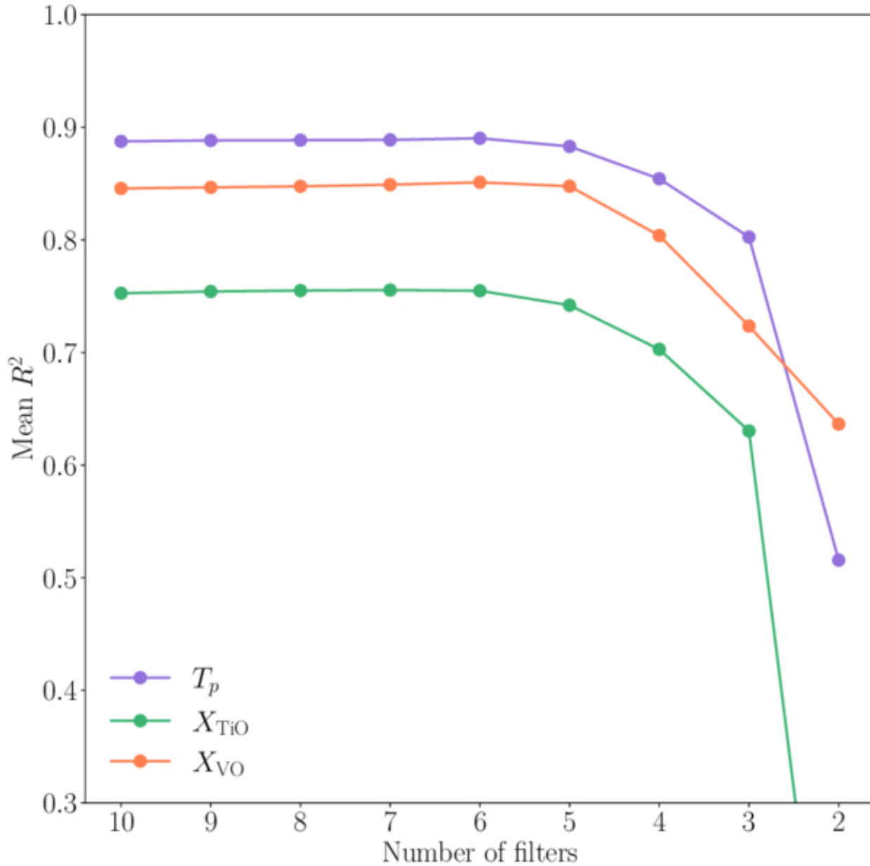
Figure 10. from Patcharawee Munsaket et al 2026 Astron. J. 172 doi:10.3847/1538-3881/ae78df https://dx.doi.org/10.3847/1538-3881/ae78df © 2026. The Author(s). Published by the American Astronomical Society.
