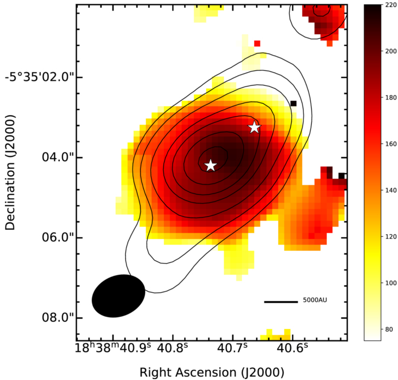
Figure 9. from Shixian Mo et al 2026 Astron. J. 172 doi:10.3847/1538-3881/ae78c8 https://dx.doi.org/10.3847/1538-3881/ae78c8 © 2026. The Author(s). Published by the American Astronomical Society.
