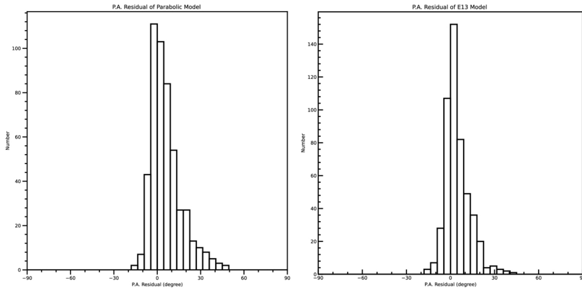
(b) Histogram of the polarization angle residuals
