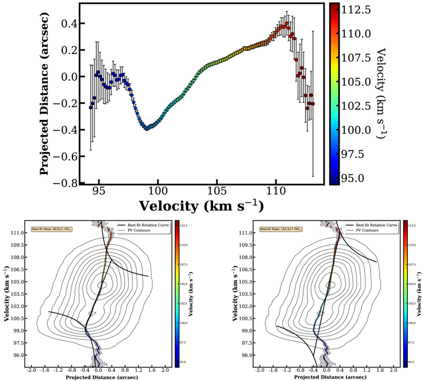
Figure 6. from Shixian Mo et al 2026 Astron. J. 172 doi:10.3847/1538-3881/ae78c8 https://dx.doi.org/10.3847/1538-3881/ae78c8 © 2026. The Author(s). Published by the American Astronomical Society.
