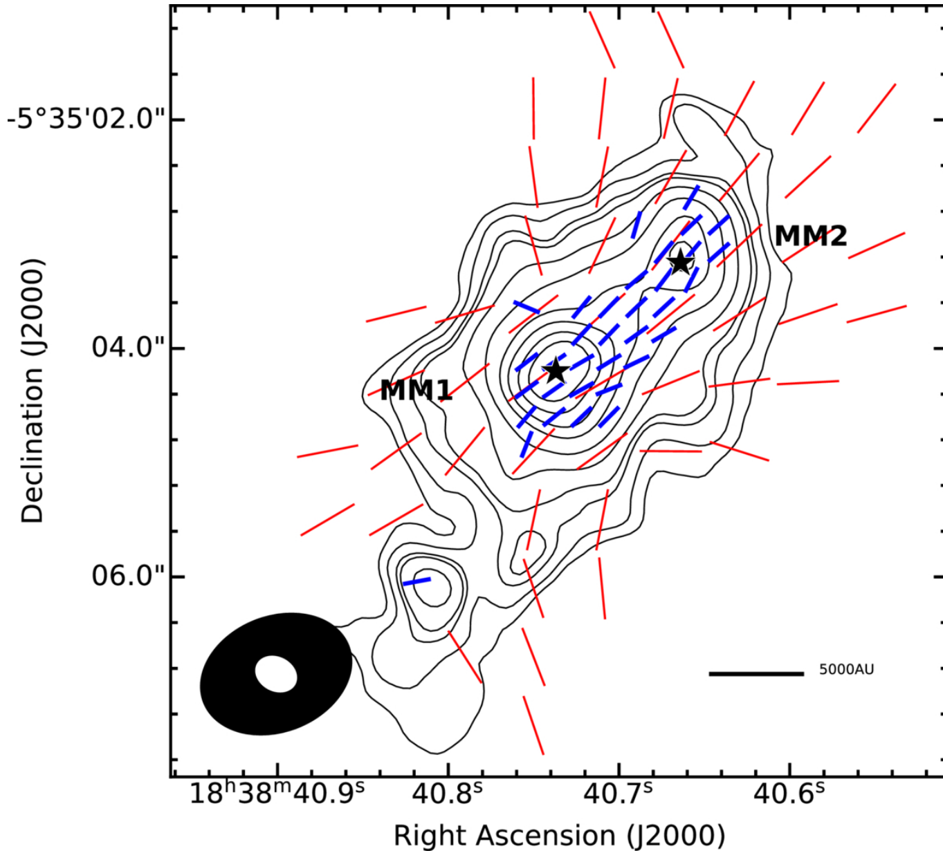
Figure 2. from Shixian Mo et al 2026 Astron. J. 172 doi:10.3847/1538-3881/ae78c8 https://dx.doi.org/10.3847/1538-3881/ae78c8 © 2026. The Author(s). Published by the American Astronomical Society.
