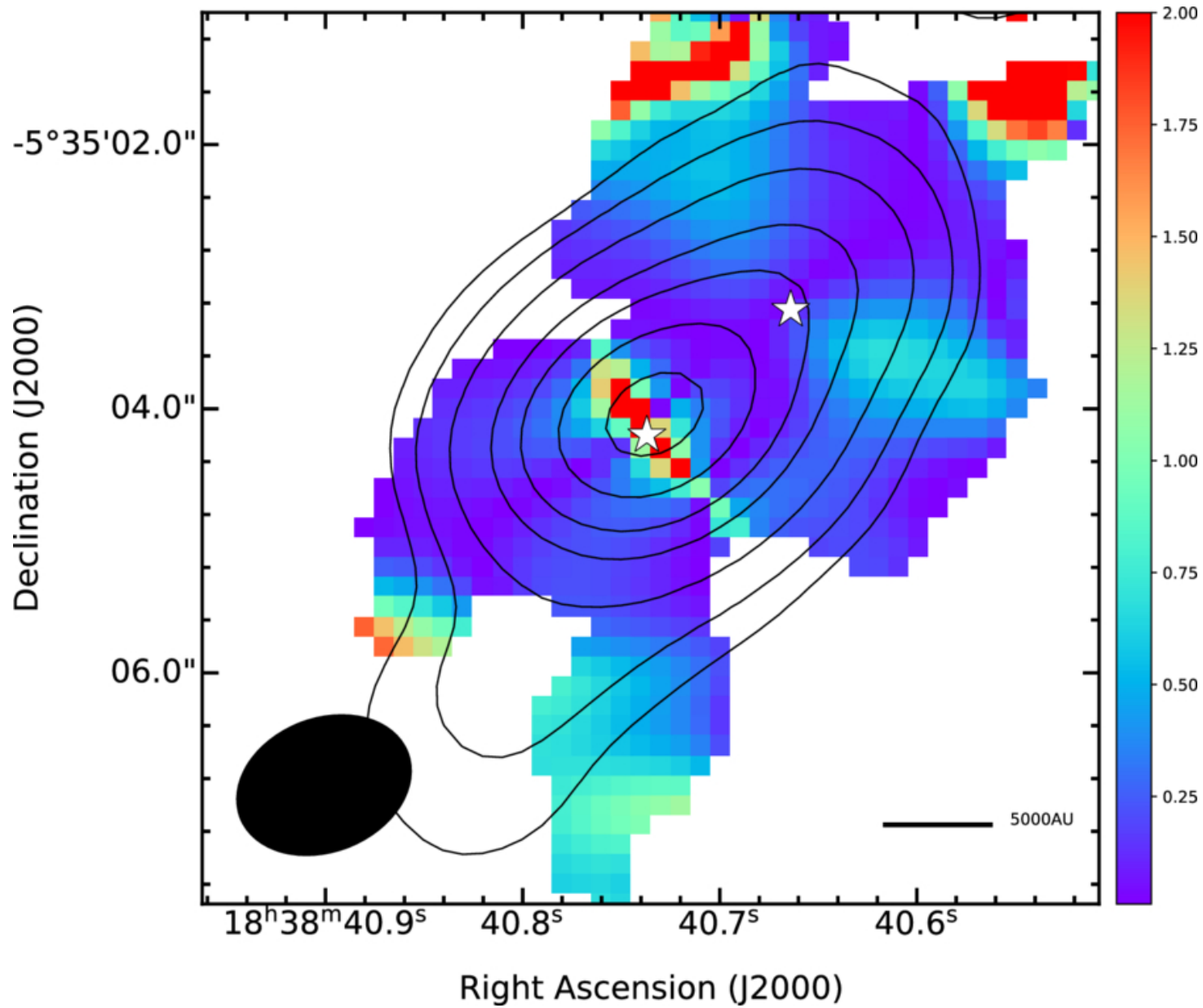
Figure 10. from Shixian Mo et al 2026 Astron. J. 172 doi:10.3847/1538-3881/ae78c8 https://dx.doi.org/10.3847/1538-3881/ae78c8 © 2026. The Author(s). Published by the American Astronomical Society.
