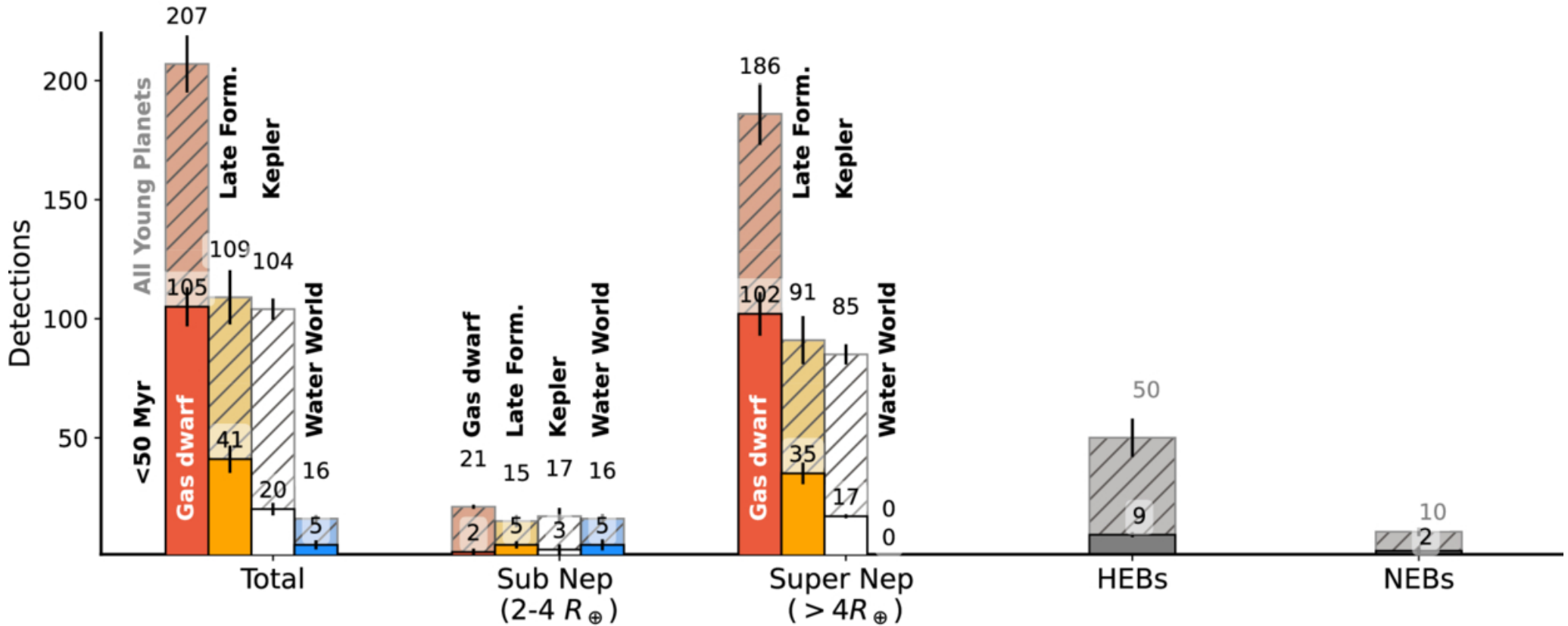
Figure 9. from George Zhou et al 2026 Astron. J. 172 doi:10.3847/1538-3881/ae7721 https://dx.doi.org/10.3847/1538-3881/ae7721 © 2026. The Author(s). Published by the American Astronomical Society.
