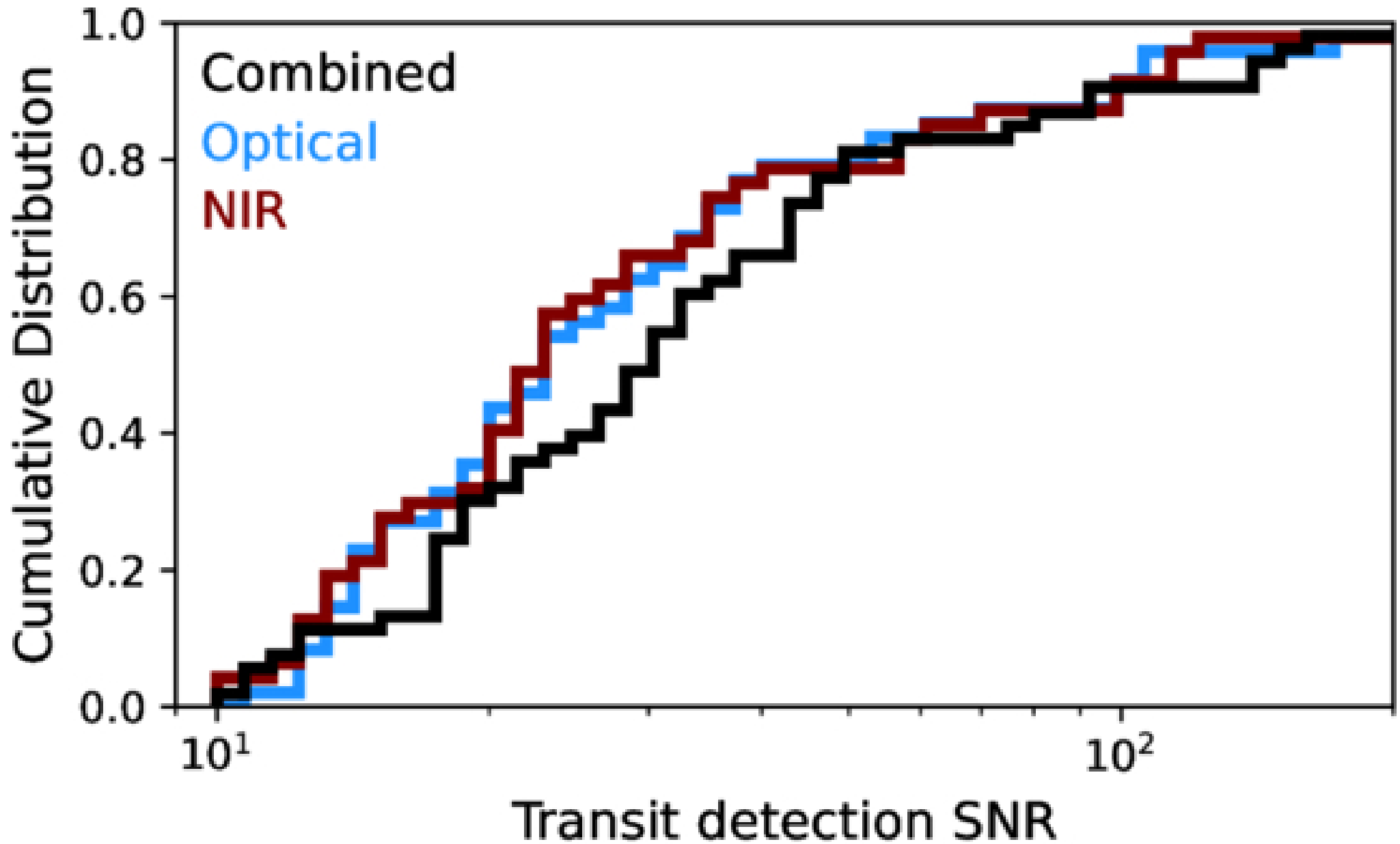
Figure 8. from George Zhou et al 2026 Astron. J. 172 doi:10.3847/1538-3881/ae7721 https://dx.doi.org/10.3847/1538-3881/ae7721 © 2026. The Author(s). Published by the American Astronomical Society.
