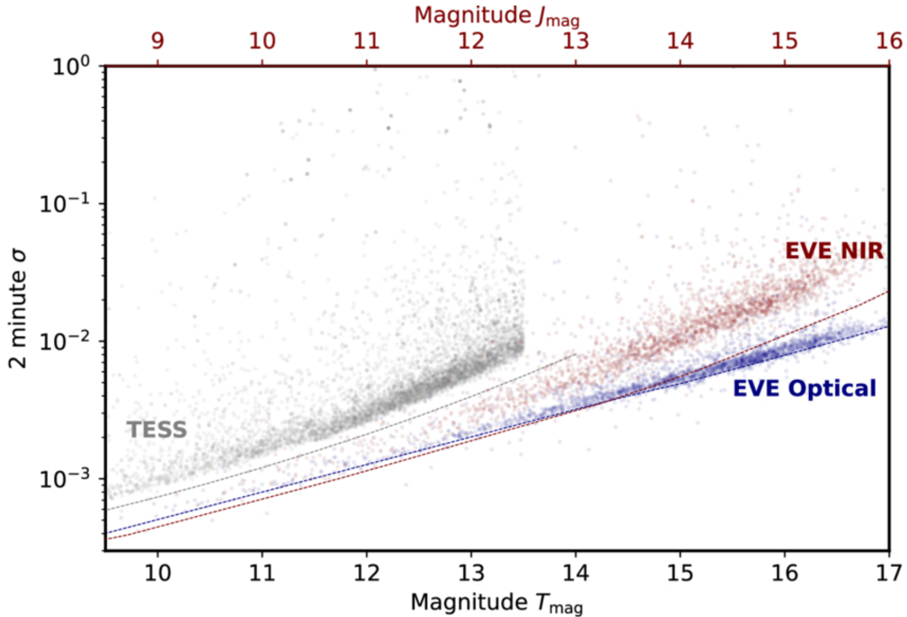
Figure 5. from George Zhou et al 2026 Astron. J. 172 doi:10.3847/1538-3881/ae7721 https://dx.doi.org/10.3847/1538-3881/ae7721 © 2026. The Author(s). Published by the American Astronomical Society.
