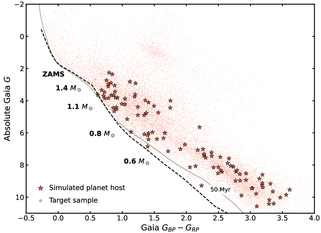
Figure 3. from George Zhou et al 2026 Astron. J. 172 doi:10.3847/1538-3881/ae7721 https://dx.doi.org/10.3847/1538-3881/ae7721 © 2026. The Author(s). Published by the American Astronomical Society.
