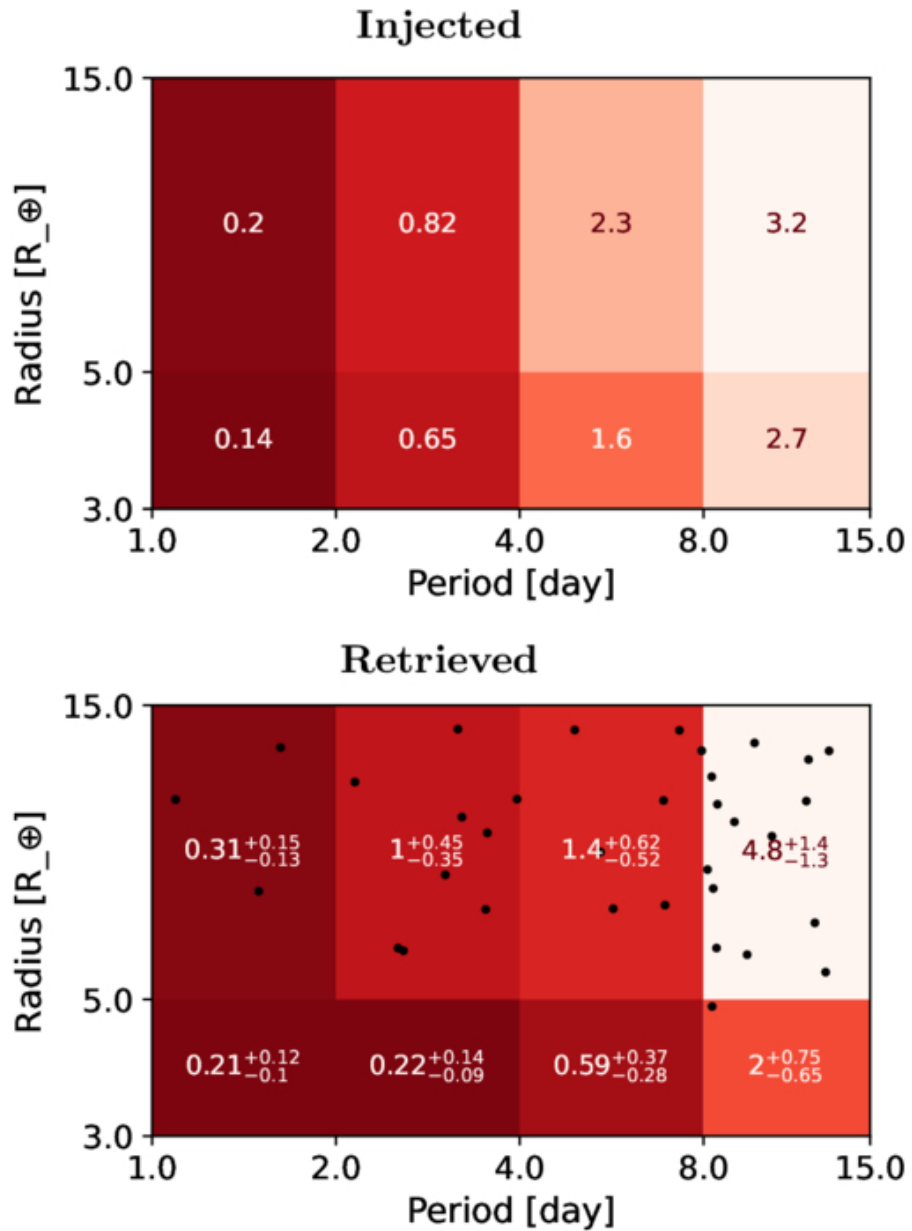
Figure 13. from George Zhou et al 2026 Astron. J. 172 doi:10.3847/1538-3881/ae7721 https://dx.doi.org/10.3847/1538-3881/ae7721 © 2026. The Author(s). Published by the American Astronomical Society.
