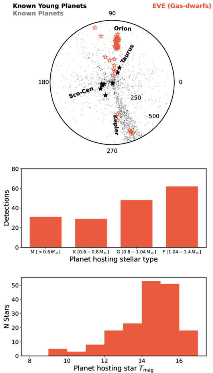
Figure 11. from George Zhou et al 2026 Astron. J. 172 doi:10.3847/1538-3881/ae7721 https://dx.doi.org/10.3847/1538-3881/ae7721 © 2026. The Author(s). Published by the American Astronomical Society.
