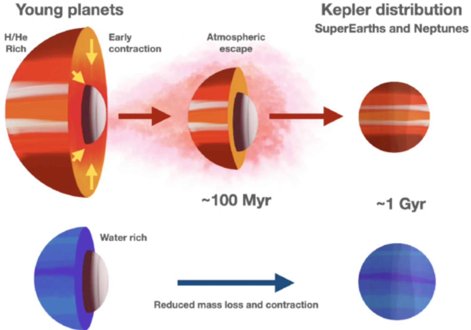
Figure 1. from George Zhou et al 2026 Astron. J. 172 doi:10.3847/1538-3881/ae7721 https://dx.doi.org/10.3847/1538-3881/ae7721 © 2026. The Author(s). Published by the American Astronomical Society.
